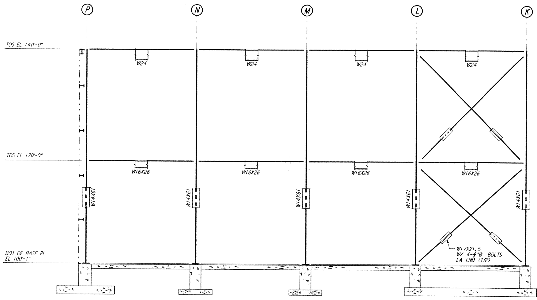
PARTIAL ELEVATION AT COLUMN LINE 8 \frac{3}{8}'' = 1'-0''
