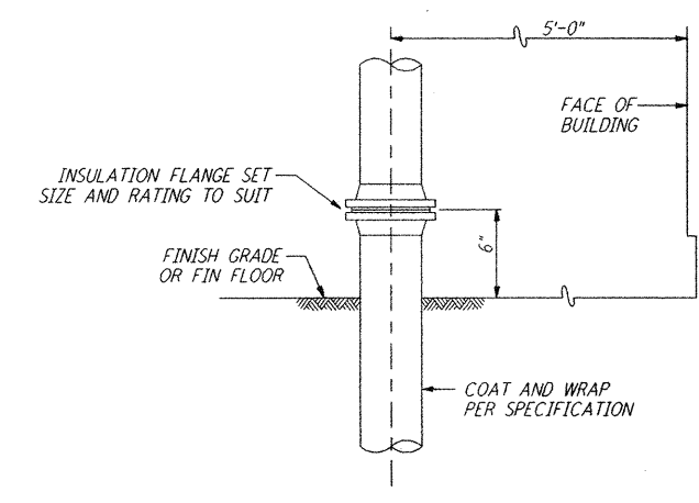
PIPE CONNECTION (4) WA-C-010 (UNDERGROUND TO OVERHEAD) NOT TO SCALE
