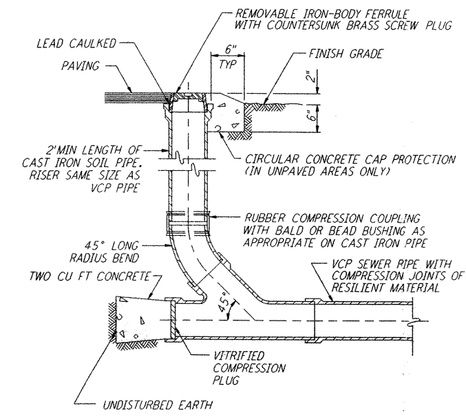
SANITARY SEWER CLEANOUT (3) WA-C-010 NOT TO SCALE
