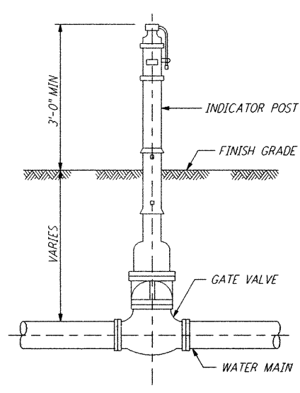
POST INDICATOR VALVE (1) WA-C-010 NOT TO SCALE
