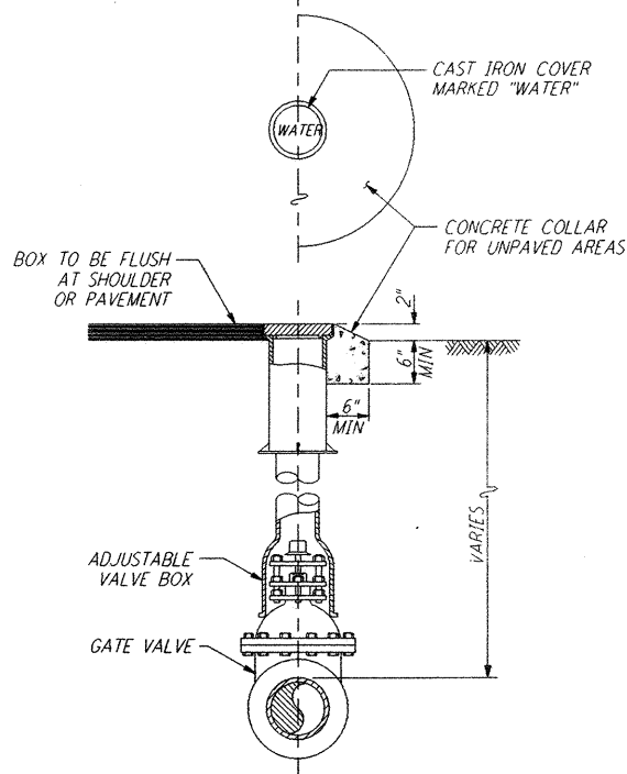
VALVE BOX (2) WA-C-010 NOTE: VALVE SIZE 12" MAXIMUM NOT TO SCALE
