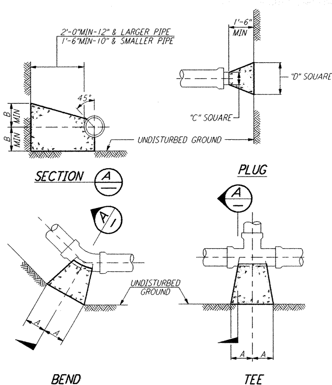
THRUST BLOCK (5) WA-C-010 NOT TO SCALE
