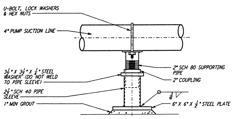
PIPE SUPPORT DETAIL 1 REF NTS WA-P-411
