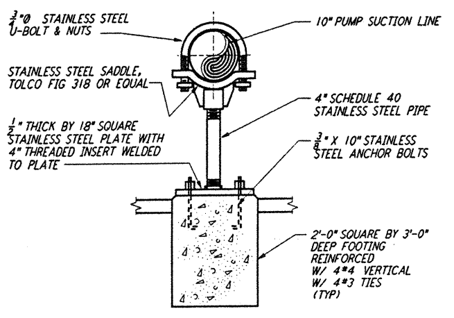
PIPE SUPPORT DETAIL 2 REF NTS WA-P-411
