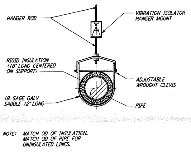
PIPE HANGER DETAIL - SINGLE PIPE 6 REF NTS WA-P-411
