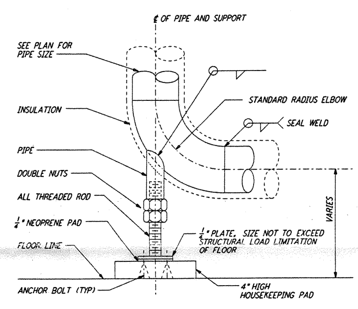
BASE ELBOW SUPPORT DETAIL 7 REF NTS WA-P-411
