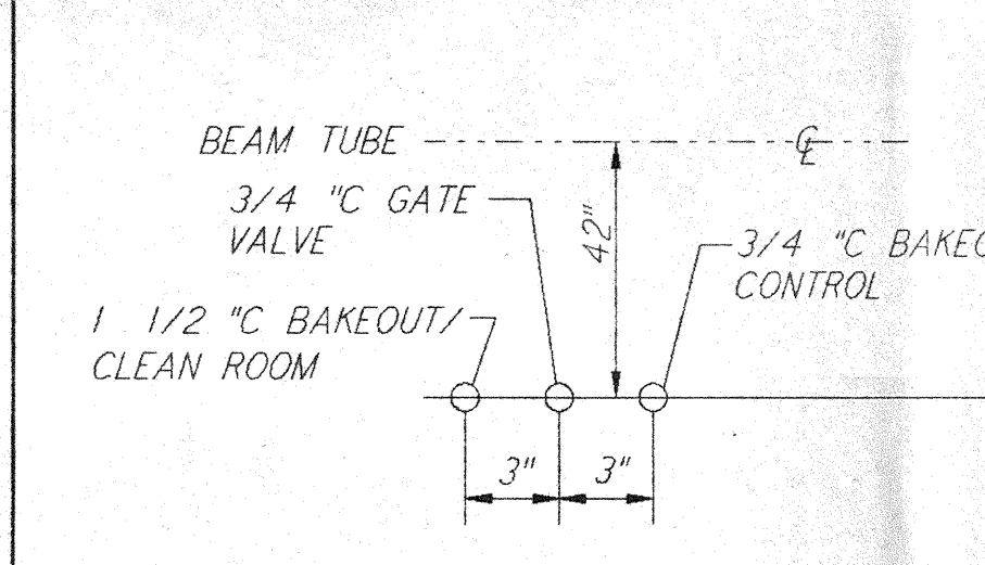
DETAIL 10 REF NTS WA-E-503
