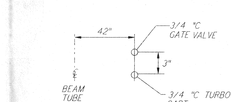
DETAIL 15 REF NTS WA-E-503
