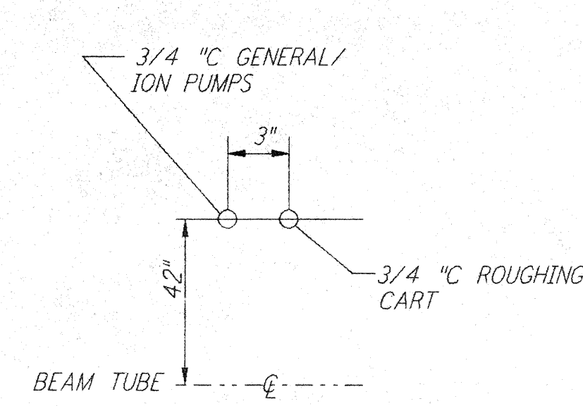
DETAIL 3 REF NTS WA-E-503 WA-E-504
