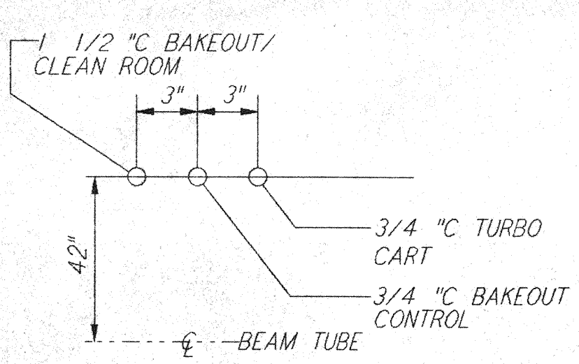
DETAIL 9 REF NTS WA-E-503 WA-E-504
