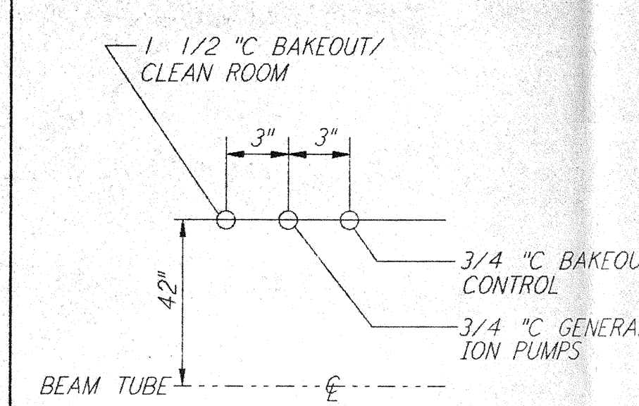
DETAIL 2 REF NTS WA-E-503 WA-E-504
