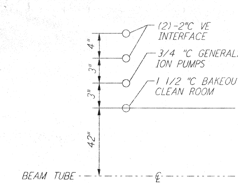
DETAIL 11 REF NTS WA-E-503 WA-E-504
