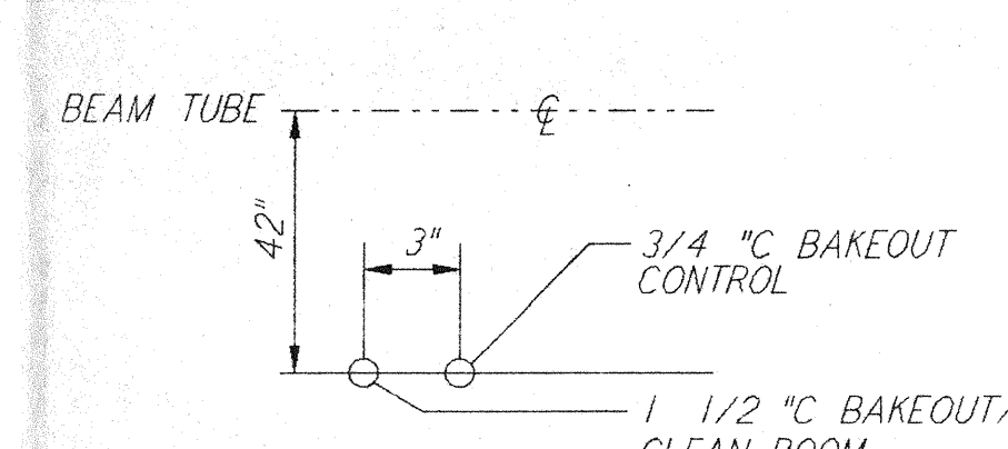
DETAIL 7 REF NTS WA-E-503 WA-E-504
