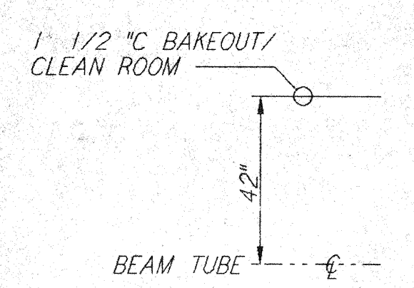
DETAIL 1 REF NTS WA-E-503 WA-E-504
