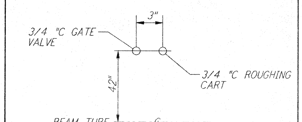
DETAIL 6 REF NTS WA-E-503 WA-E-504
