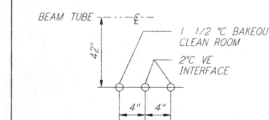
DETAIL 13 REF NTS WA-E-503 WA-E-504
