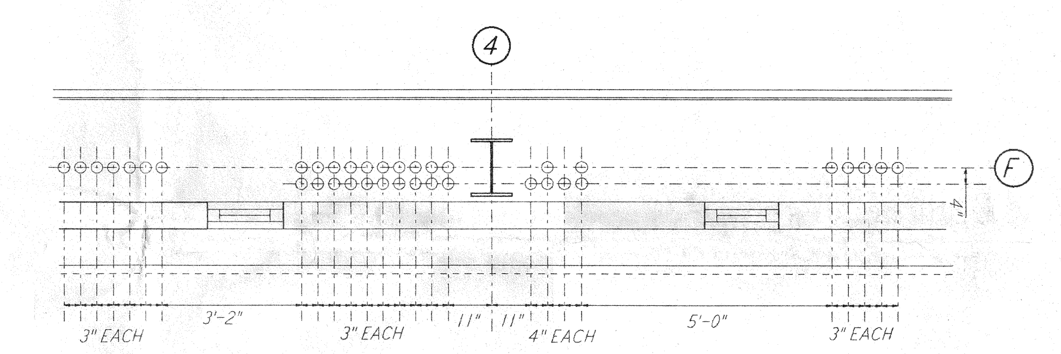
DETAIL 20 REF NTS WA-E-503
