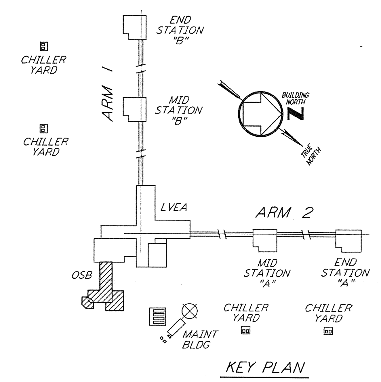
KEY PLAN 0 8 16 24 32 FT 1/8" = 1'-0"
