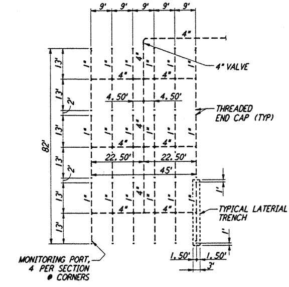
(3 SECTIONS TOTAL) TYPICAL LEACH FIELD SECTION SCALE: 1" = 20"
