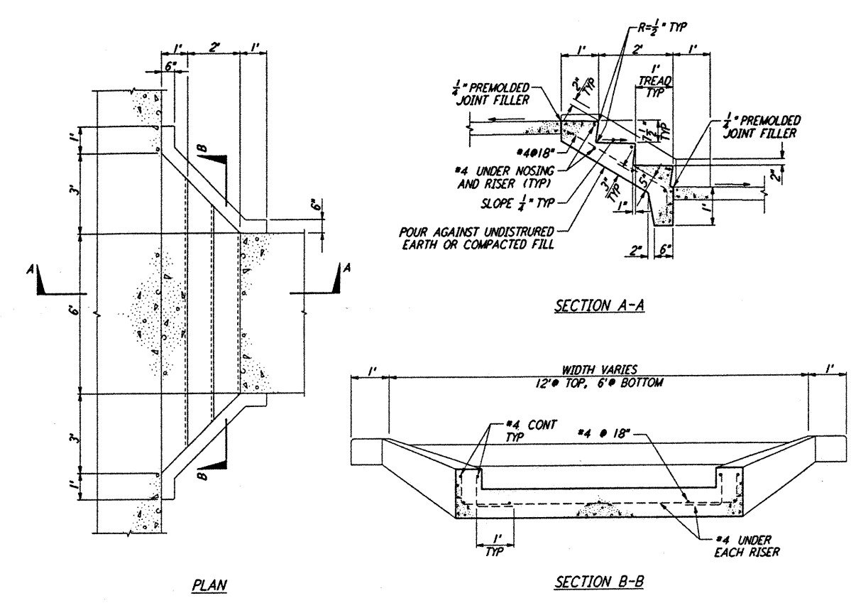
CONCRETE STEPS (1) NOT TO SCALE REF: WA-C-052, WA-C-505, WA-C-006
