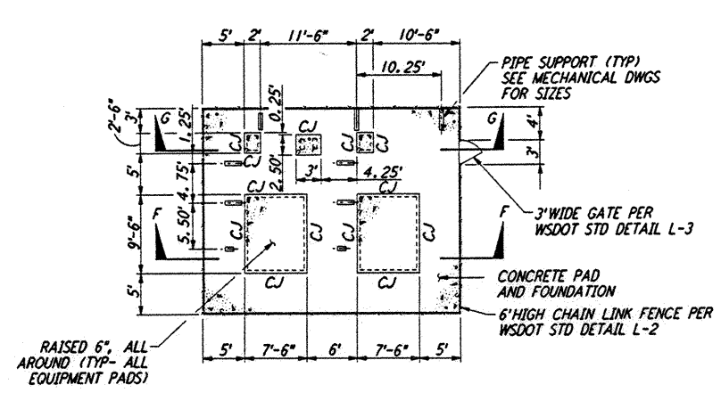
ENLARGED CHILLER YARD PLAN @ MID AND END STATIONS (3) NOT TO SCALE REF: WA-C-052, WA-C-021, WA-C-025, WA-C-041, WA-C-045 NOTE: FOR MID AND END STATIONS - NORTHWEST ARM, USE PLAN AS SHOWN. FOR MID AND END STATIONS - SOUTHWEST ARM, PLAN IS ROTATED 90° AND MIRRORED ABOUT THE BEAM TUBE.
