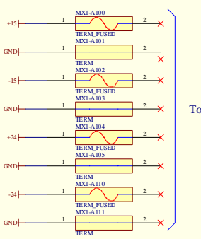
LIGO EuroCard Crate Power Connections
