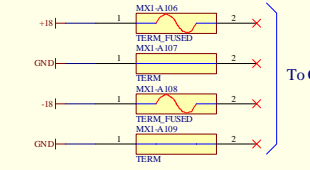
Glasgow EuroCard Crate Power Connections
