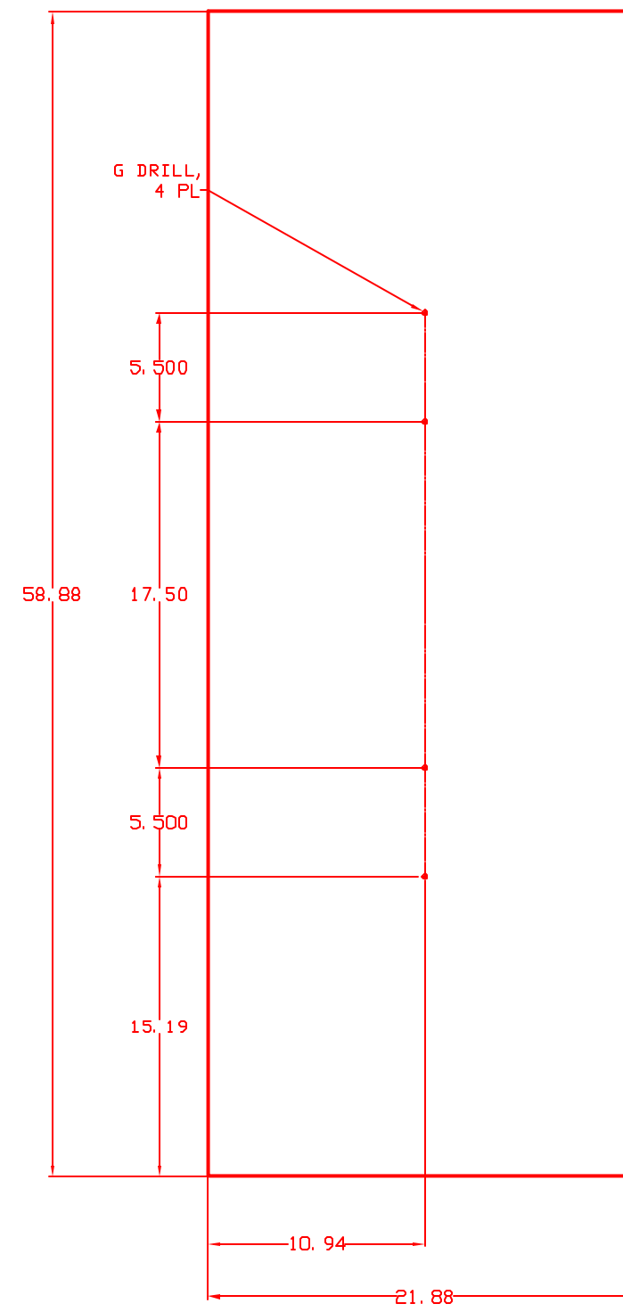
-3 22X59 LID MAT'L: 6061-T6 ALUMINUM; 2 REQ'D.
