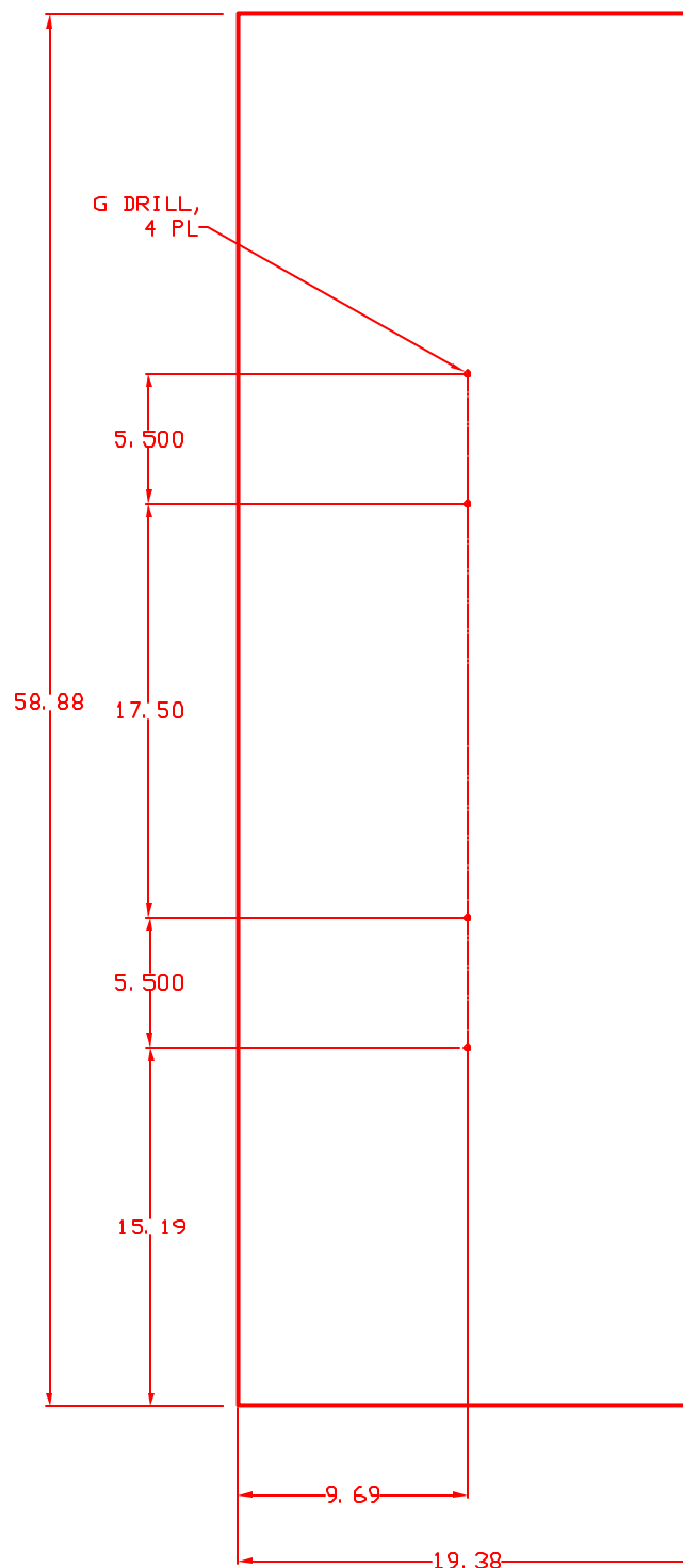
-2 20X59 LID MAT'L: 6061-T6 ALUMINUM; 5 REQ'D.
