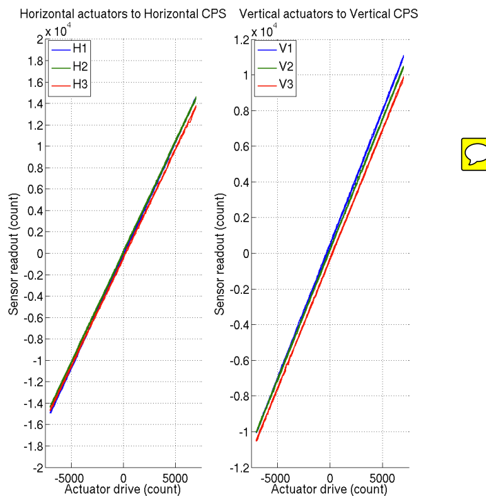
Figure - Linearity test on the triplet ‘actuators - HAM-ISI – sensors’ in both Horizontal and vertical directions
