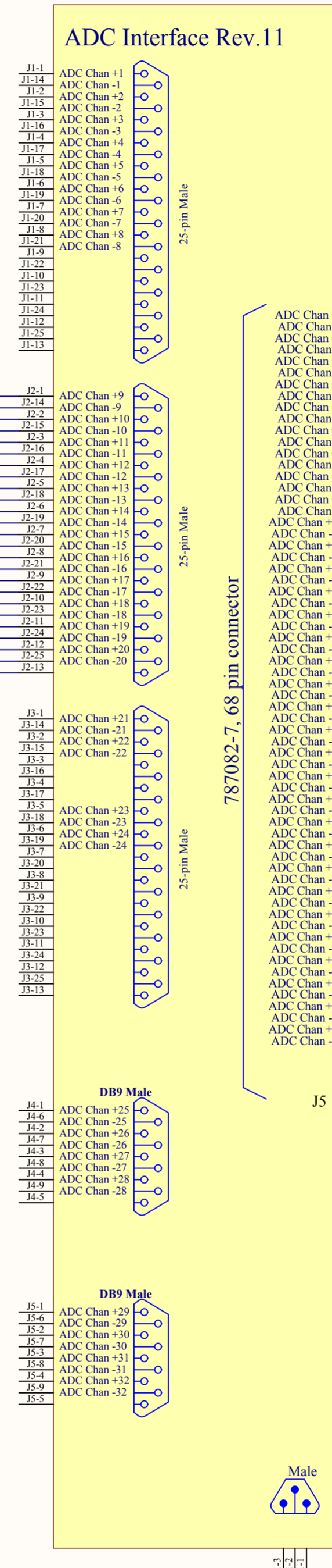
ADC Interface HAM_ISI
