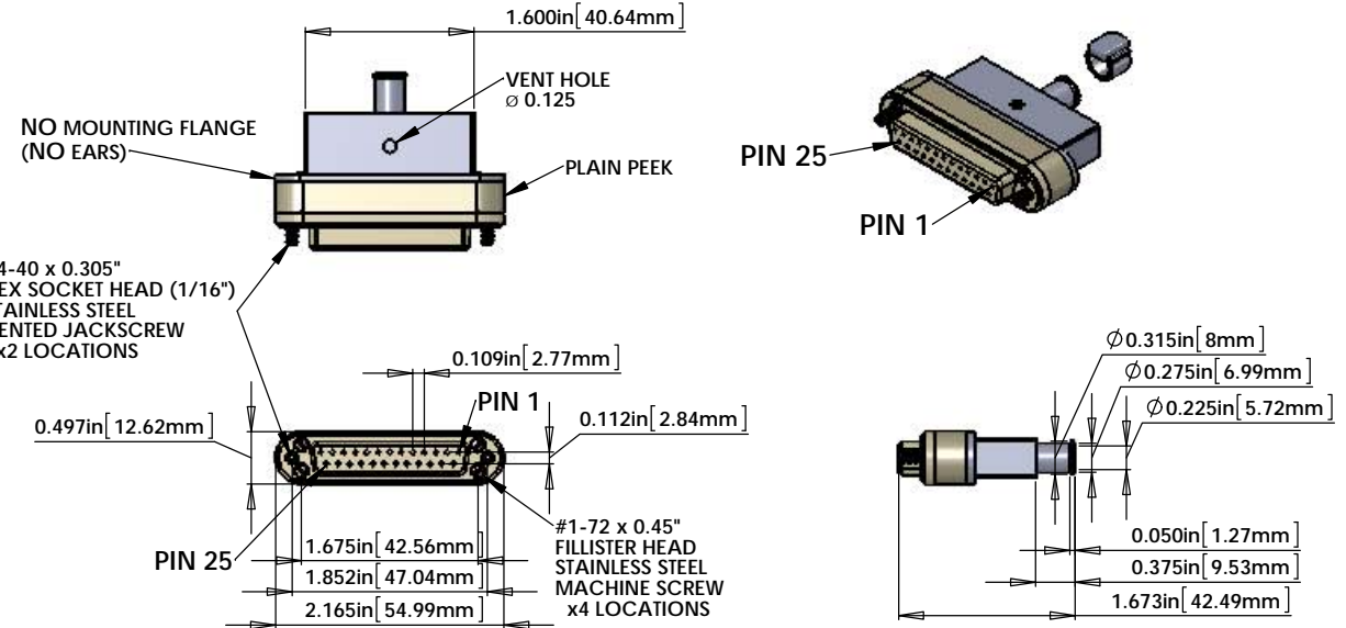
CONNECTOR J1
