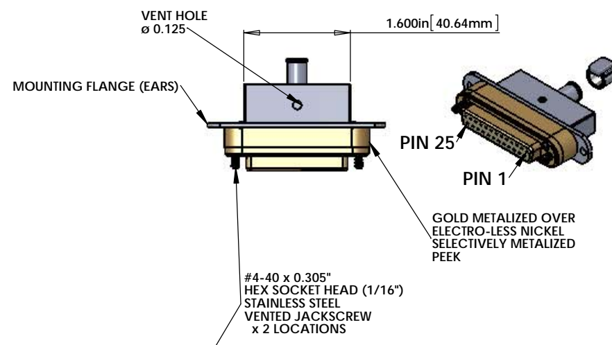
CONNECTOR J2
