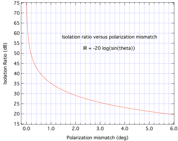
FIG. 31: Faraday isolation ratio vs polarization mismatch.
