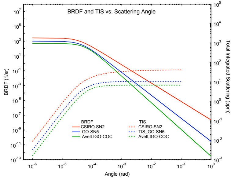
FIG. 18: BRDF functions determined from measured power spectral density data for iLIGO COC
