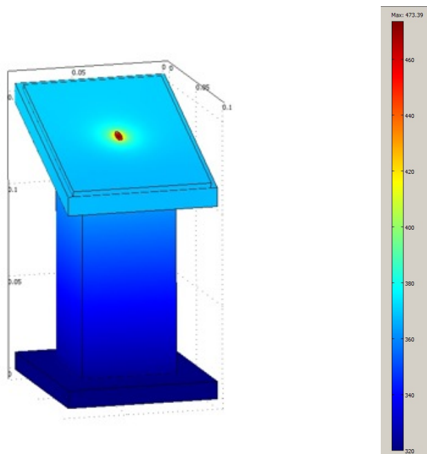
FIG. 27: Surface Temp Plot (REFL beam dump)
