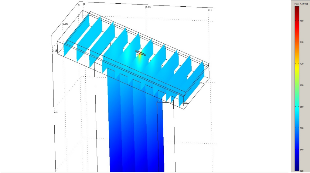
FIG. 28: Isotherm slice plot (REFL beam dump)
