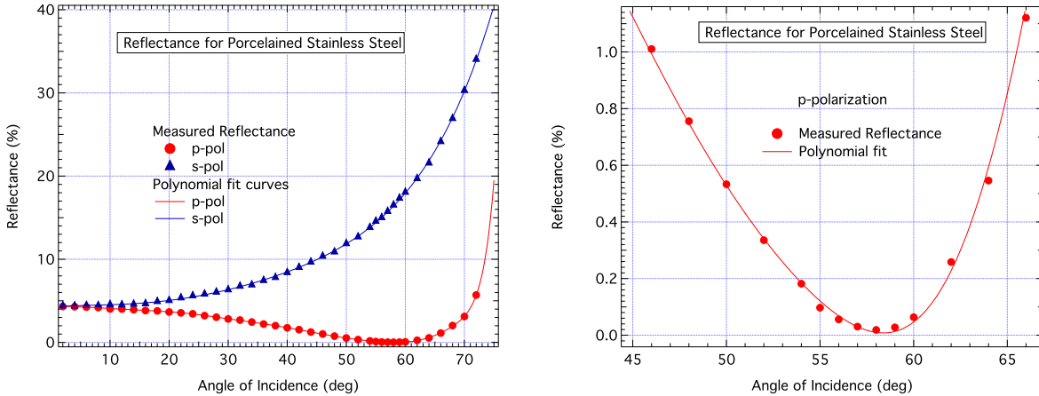
FIG. 29: Reflectivity of PSS vs AOI
