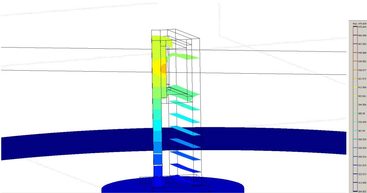
FIG. 26: Isotherm slice plot (Parking Beam Dump on HAM2 table)
