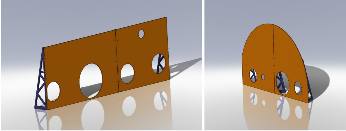
FIG. 8: HAM2 and HAM3 Table Baffles
