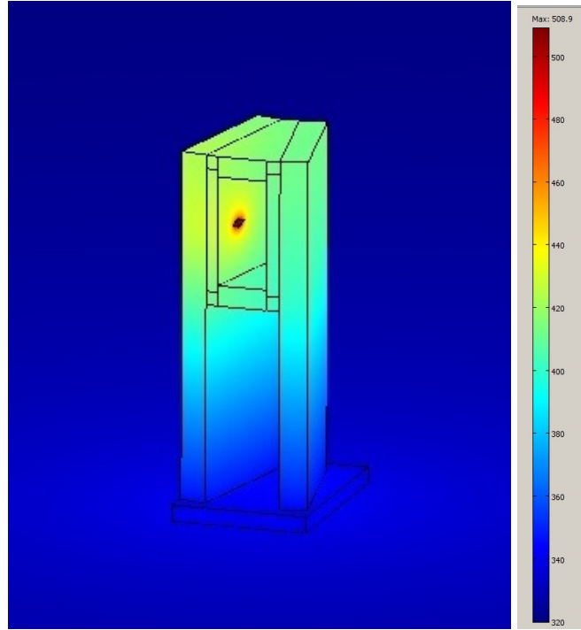
FIG. 25: Surface Temp Plot (Parking Beam Dump on HAM2 table)
