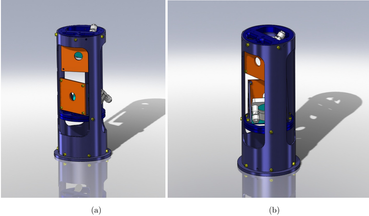
FIG. 10: MC REFL Periscope Baffles - (a) HA-7 Top/Bottom for Periscope 1, and (b) HA-8 Top/Bottom for Periscope 2
