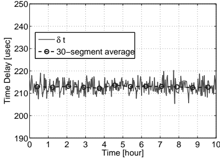
Figure 7. Simulated time delay measurement.
