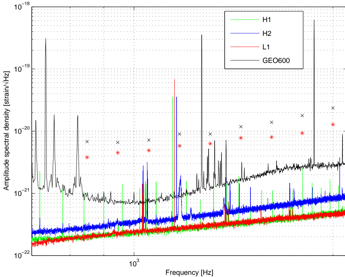
Figure 8. The h_{\text{TSS}}^{50\%} values for Waveburst-CorrPower ('x' markers) and coherent Waveburst ('*' markers) pipelines for sine-Gaussians of different central frequencies. Coherent Waveburst is sensitive to gravitational wave signals with amplitudes 30 – 50% lower than those detectable by Waveburst-CorrPower.
