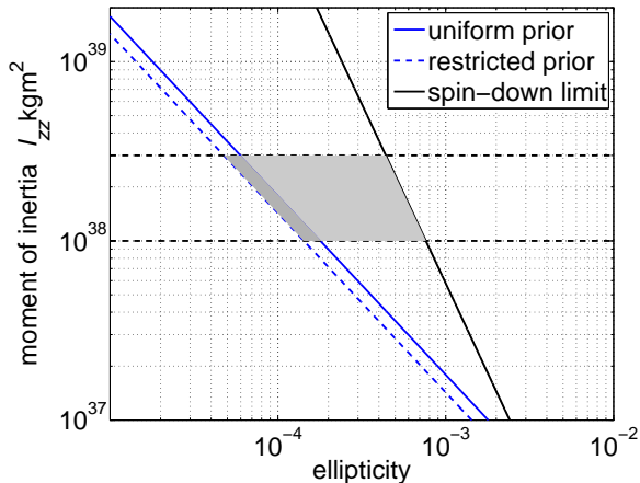
FIG. 1.— The single template search upper limits from S5, for the uniform and restricted prior ranges, and spin-down upper limit plotted as exclusion regions in a moment of inertia–ellipticity plane. Areas to the right of the diagonal lines are excluded. The dashed horizontal lines represent estimates of the theoretical lower and upper bounds of acceptable moments of inertia at 10^{38} \text{ kg m}^2 and 3 \times 10^{38} \text{ kg m}^2 . The shaded area represents the region that is newly excluded with these results.
