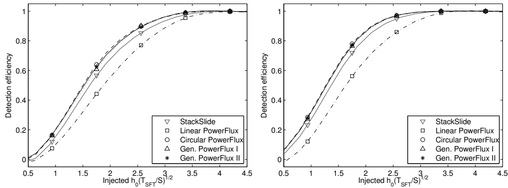
Figure 2. Same as Figure 1, for 336 (left) and 672 SFTs (right), and a signal declination of 45 degrees.
