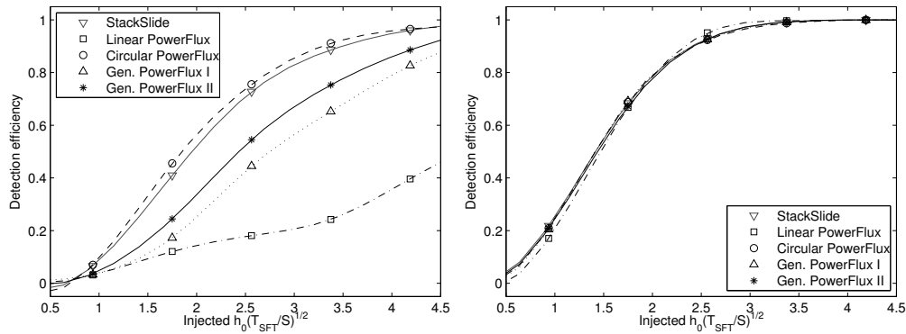
Figure 1. Detection efficiency versus the normalized injected amplitude, for 336 SFTs and signal declinations of zero (left) and 90 degrees (right). The marked points are the results of the simulated searches. The solid lines are spline fits to the marked points; errors in these fits are less than 3%.
