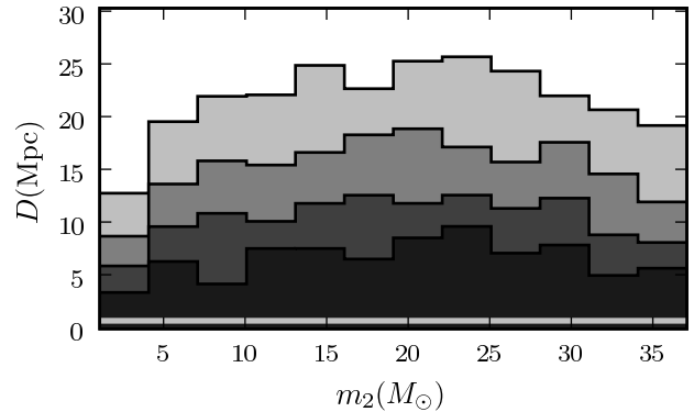
FIG. 3.— The probability as described in eq. (3) computed using the loudest event method where the injections are made only into the 180 s segments immediately before and after the on-source time. The shaded regions represent 90%, 75%, 50%, and 25% exclusion regions, from darkest to lightest respectively. The distance to M31 is indicated by the horizontal line at D = 0.77 Mpc. Both amplitude calibration uncertainty and Monte-Carlo statistics are included in this result; apparent fluctuations as a function of mass are due to Monte Carlo uncertainty.
