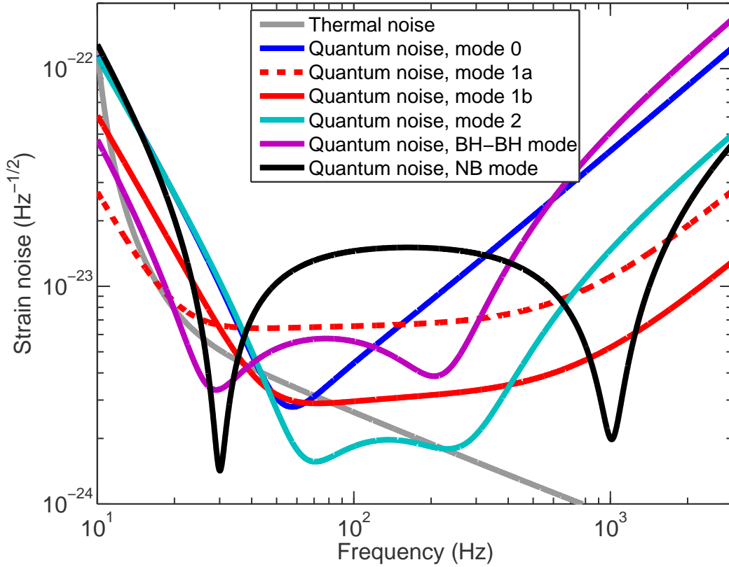
Figure 4: Quantum noise for the modes described in Section 3.1, as well as two additional modes (of more specialized interest): a mode tuned for detection of an inspiral of two 30-solar-mass black holes (BH-BH); a narrowband mode where the signal recycling mirror is changed for one with much smaller transmission (1.1% vs. 20%). Total thermal noise (suspension and test mass) is also shown for comparison.
