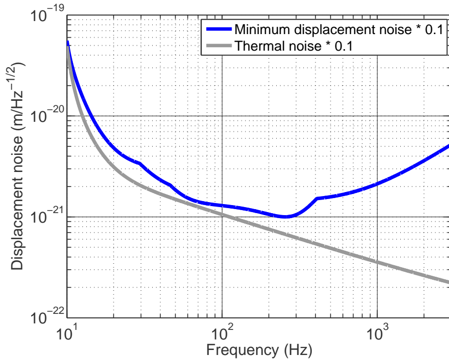
Figure 6: Equivalent differential-arm displacement noise limit for technical noise sources. The blue curve is 10% of the minima of the curves shown in Fig. 2 (converted to displacement by multiplying by the arm length). Displacement noise limit for a single test mass would be a factor of 2 smaller. For reference, the grey curve is 10% of the thermal noise (sum of suspension and test mass internal noise).
