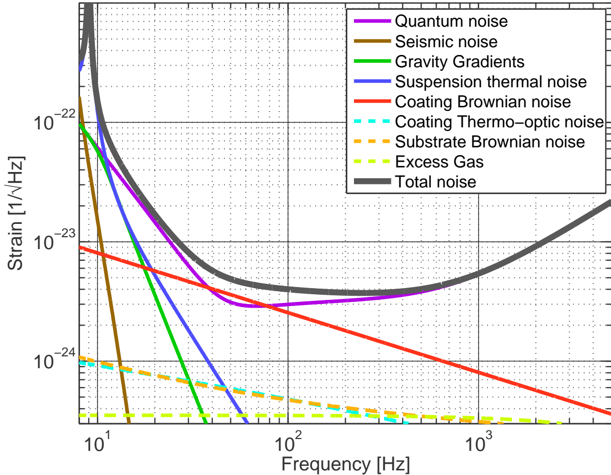
Figure 3: Fundamental noise sources for broadband, high power operation—mode 1b of Fig. 2, with 125 W of input power.
