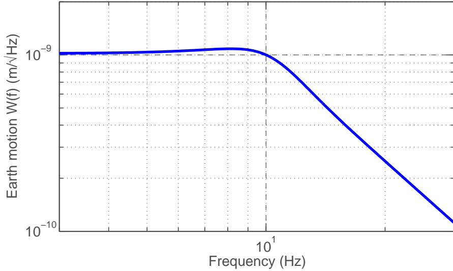
Figure 5: Model used for the rms seismic displacement in the gravity-gradient noise estimate, averaged over horizontal and vertical directions (the motion spectrum W(f) as defined in Ref. [59]).
