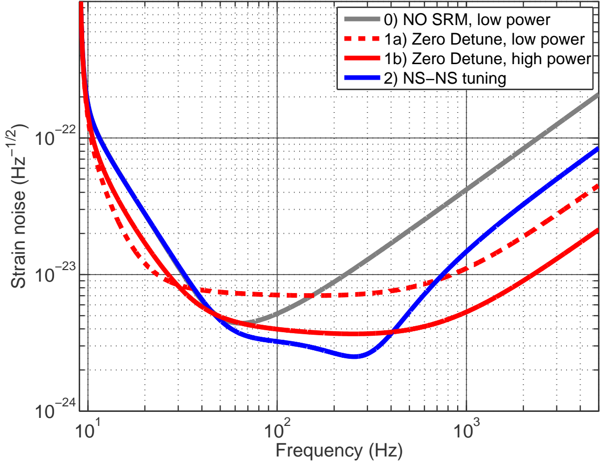
Figure 2: Likely modes of operation for the Advanced LIGO interferometers. See text for description of the modes.
