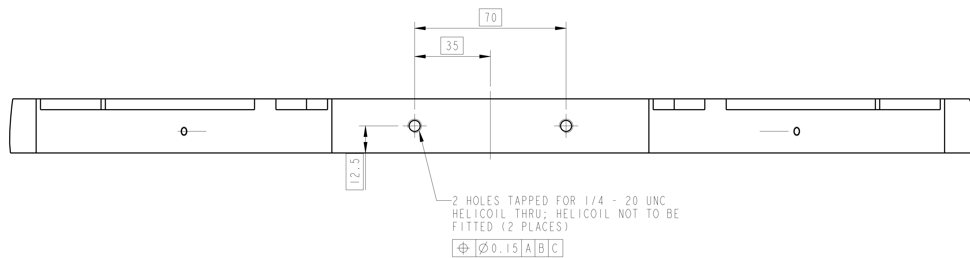
DETAIL R (SEE SHT 1) SCALE 1:1
