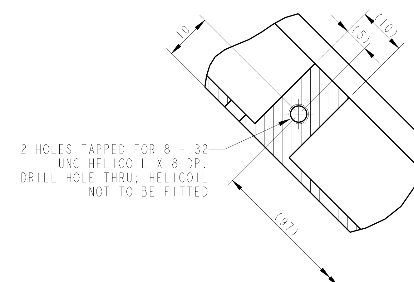
PARTIAL SECTION U-U SHOWING HOLE POSITION (TYP 2 PLACES)
