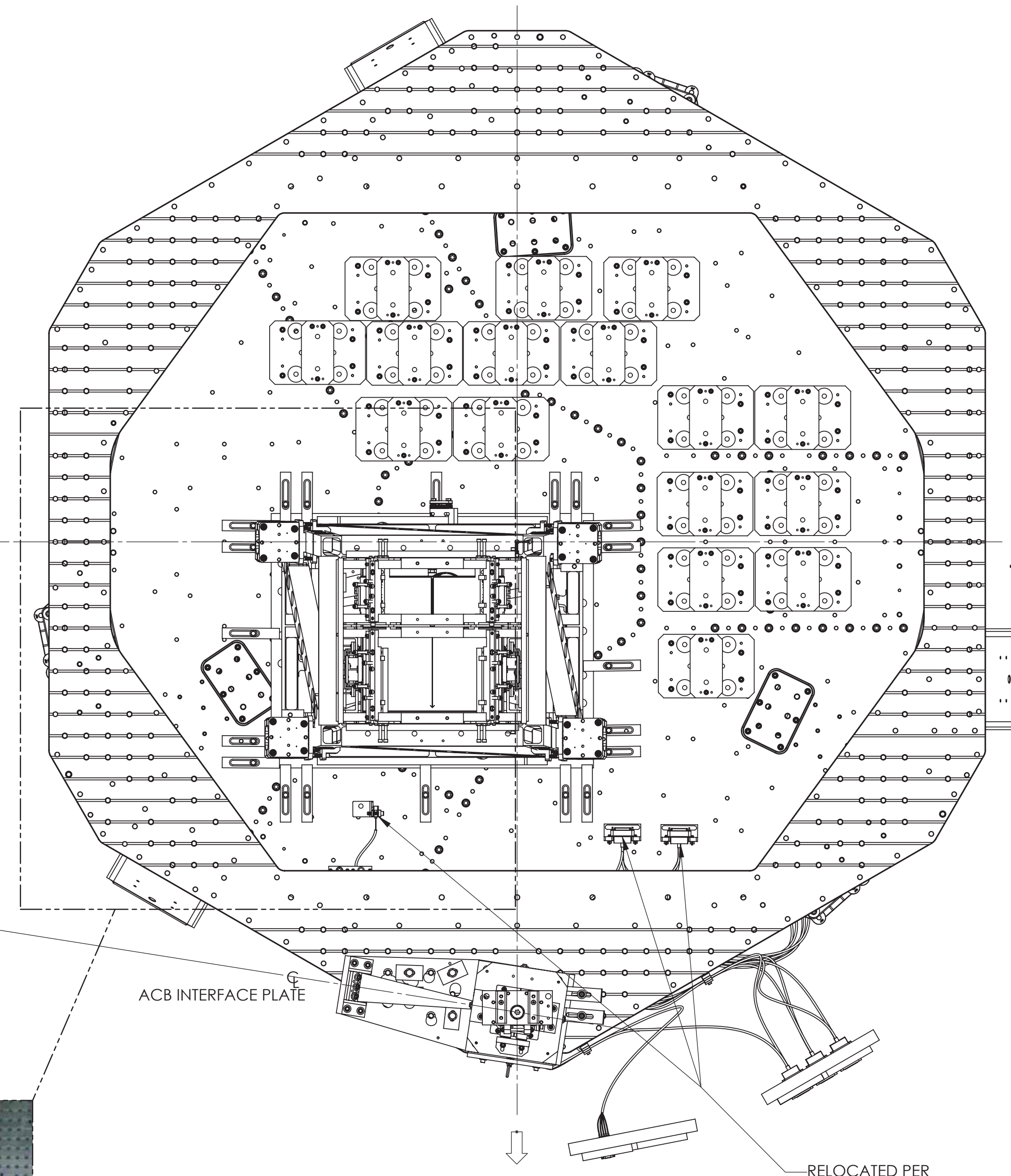
BOTTOM VIEW ACB BOX NOT SHOWN FOR CLARITY (LOOKING UP)
