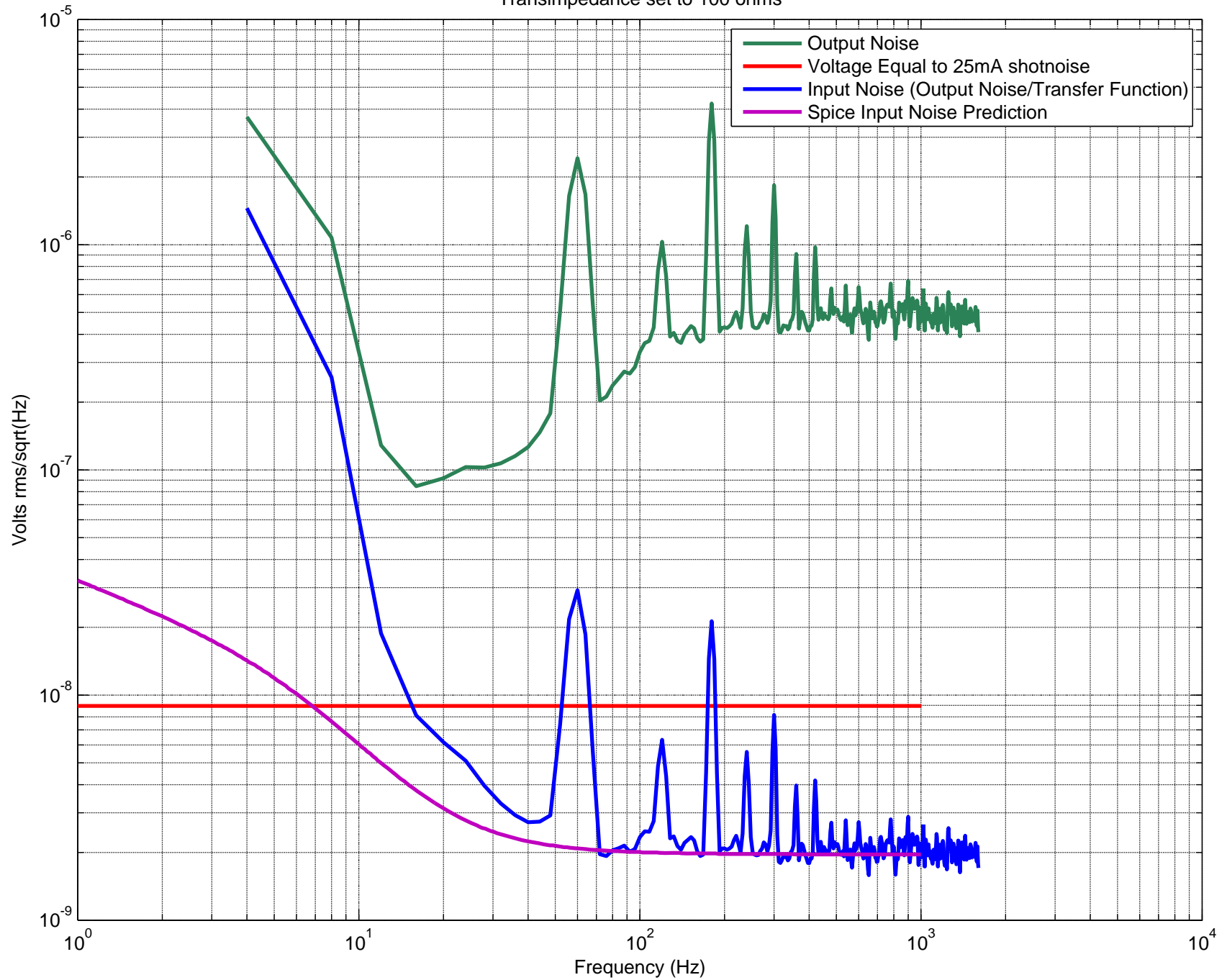
ELIGO OMC In-vacuum DCPD SN002 Voltage Noise Transimpedance set to 100 ohms
